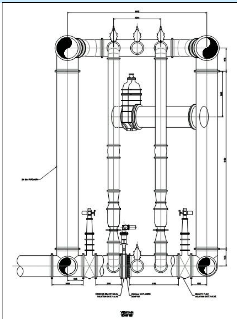
Station Arrangement
