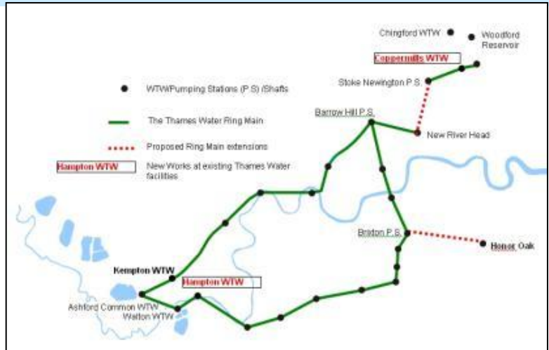
The Thames Water Ring Main
